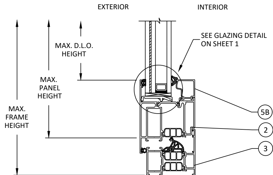
D 4 VERTICAL SECTION TYP. SILL DETAIL
