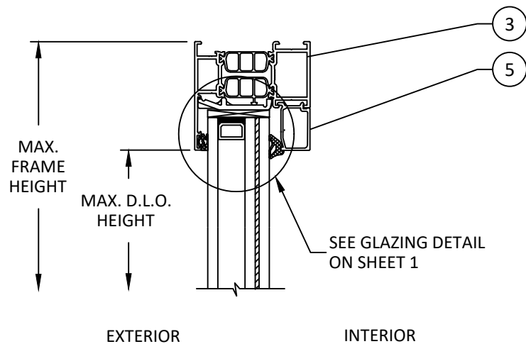
A 4 VERTICAL SECTION TYP. HEAD DETAIL
