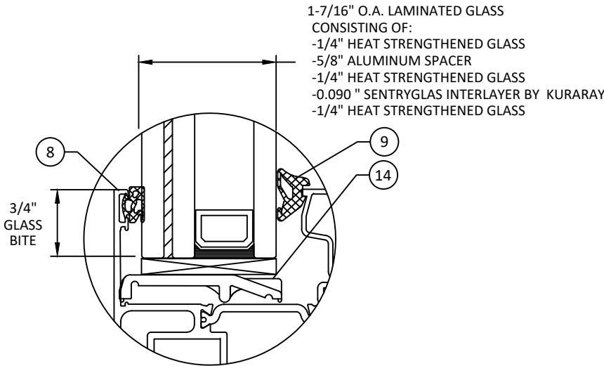
GLAZING DETAIL 1
