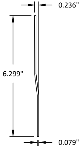
6 INSTALLATION FIN CARBON GALVANIZED STEEL
